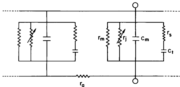
FIGURE 1 The model cable used in the calculations. The values used for the calculations were R_m = 1,500 \text{ ohm cm}^2 , R_s = 600 \text{ ohm cm}^2 , R_a = 170 \text{ ohm cm} , c_m = 1 \times 10^{-6} \text{ F/cm}^2 , and C_t = 6 \times 10^{-6} \text{ F/cm}^2 . The fiber radius, a , was taken as 30 \times 10^{-4} \text{ cm} . Then r_m = R_m/2 \cdot \pi \cdot a ; r_a = R_a/\pi \cdot a^2 ; r_s = R_s/2 \cdot \pi \cdot a ; c_m = C_m \cdot 2 \cdot \pi \cdot a ; c_t = C_t \cdot 2 \cdot \pi \cdot a . Values for r_j were calculated as described in the text.
