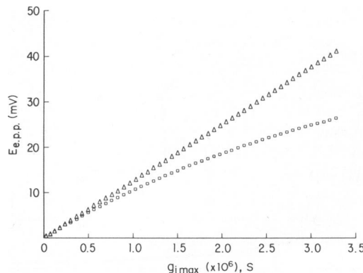
FIGURE 7 The peak epps calculated from the diffuse end-plate model ( \square ), along with the correction by Martin's method ( \diamond ). The correction is excellent.
