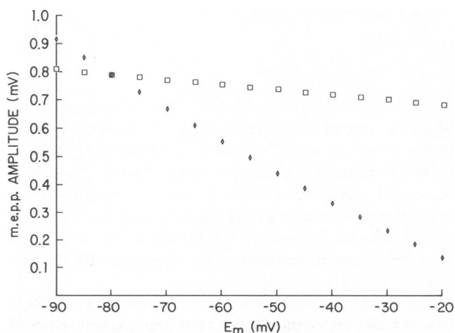
FIGURE 8 \diamond , peak amplitudes of modeled miniature end-plate potentials. \square , amplitudes corrected by the method of Katz and Thesleff (1957) for a potential of -80 mV; m.e.p.p. , miniature end-plate potential.
